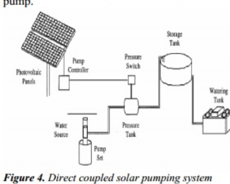
Figure 4. Direct coupled solar pumping system [5]
